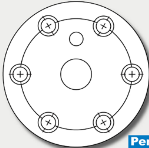
Long Year Bolt Hole Patern - P5
